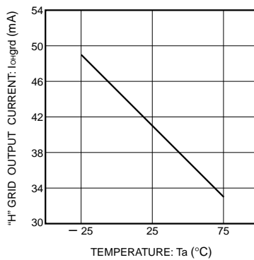
Fig. 6 "H" grid output current temperature characteristics
